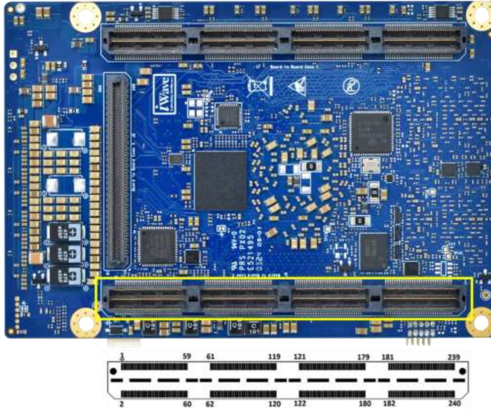
Board to Board Connector1 (J6)
