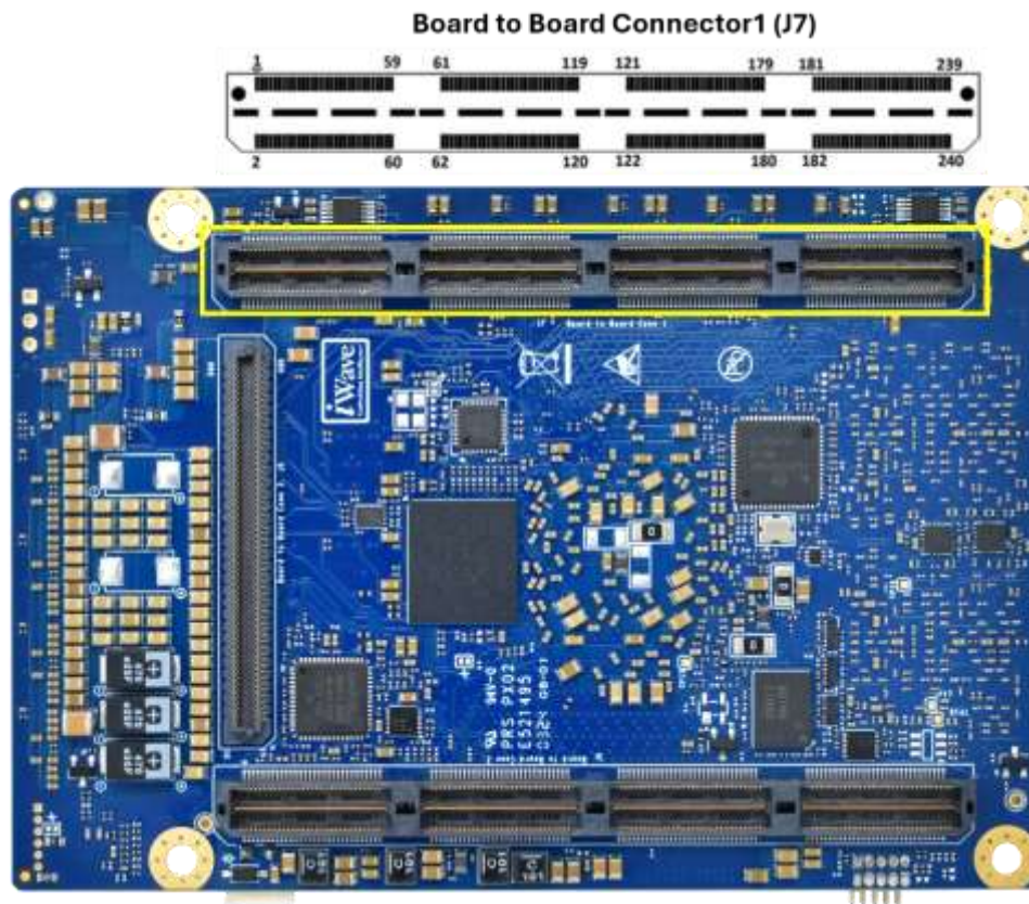
Figure 6: Board-to-Board Connector1
