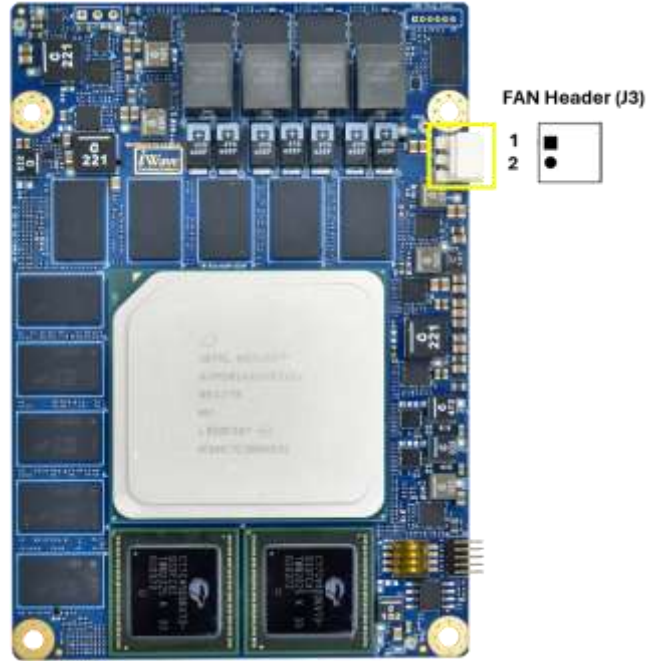
Figure 5: Fan Header
